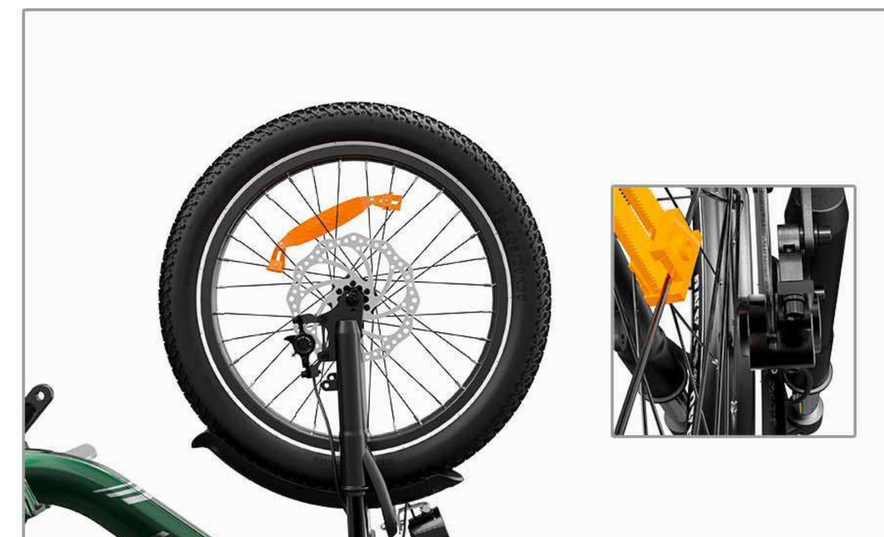
09 Put the wheel in the front fork Disc brake disc alignment clamp card slot
