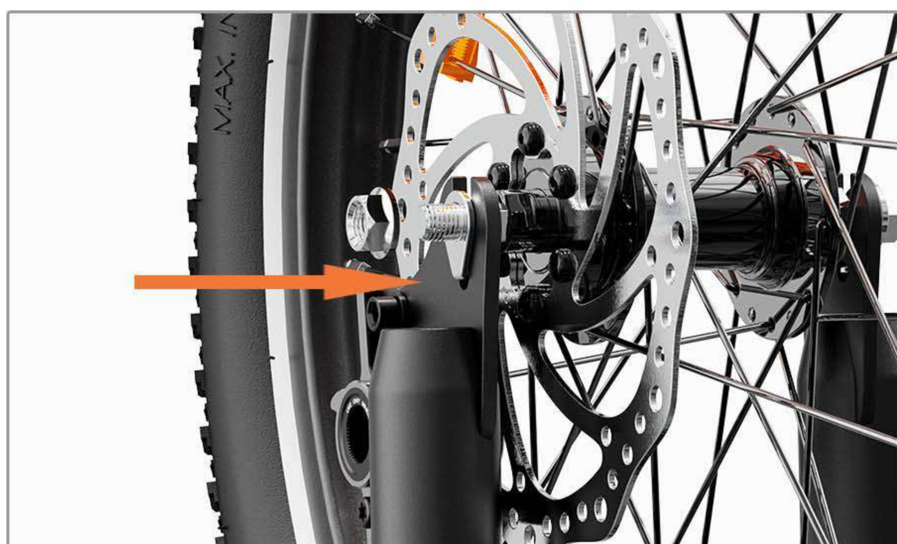
10 Install buckles and large nuts on both sides at the same time The buckle needs to snap into the installation hole
